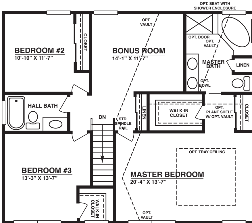
OPTIONAL 4-BEDROOM EXPANDED SECOND FLOOR PLAN
